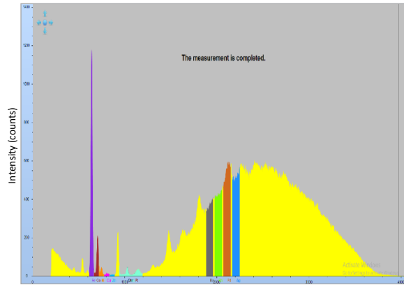
EDXRF
