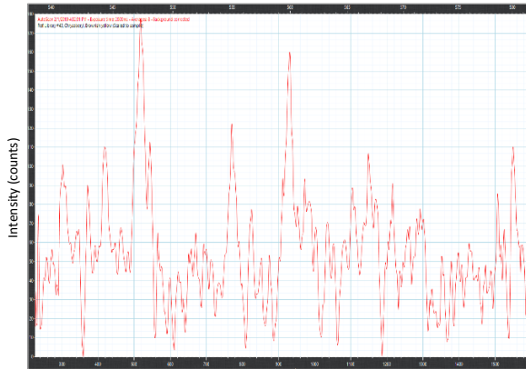
RAMAN
