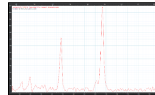
RAMAN
